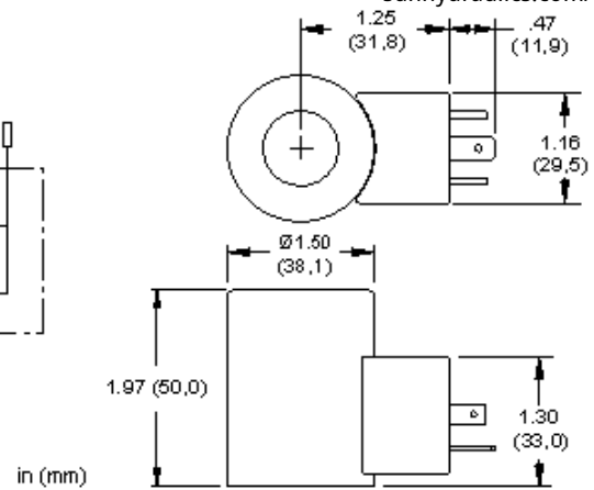
DC COIL
